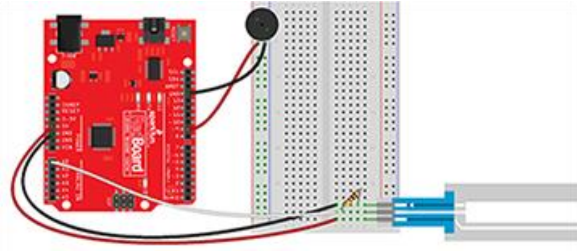
Figure 2. A wiring schematic of the keyboard.
