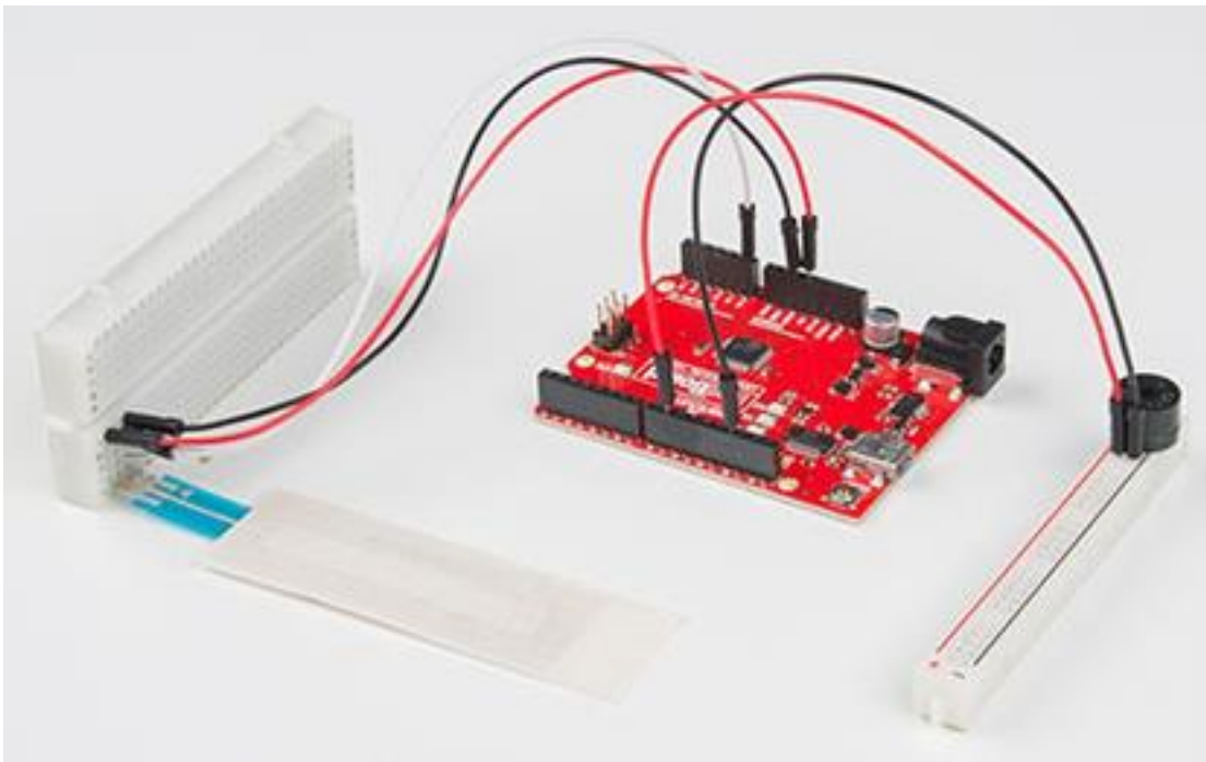
Figure 3. An assembled keyboard with cut breadboard.
